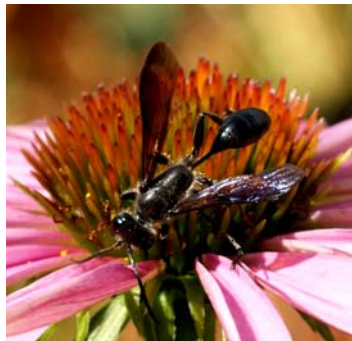
Grass Carrying Wasp, Isodontia mexicana
